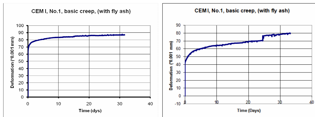
Fig. 1: Basic creep of dried specimens (left – in 5 months age, right – in 1 month age).
