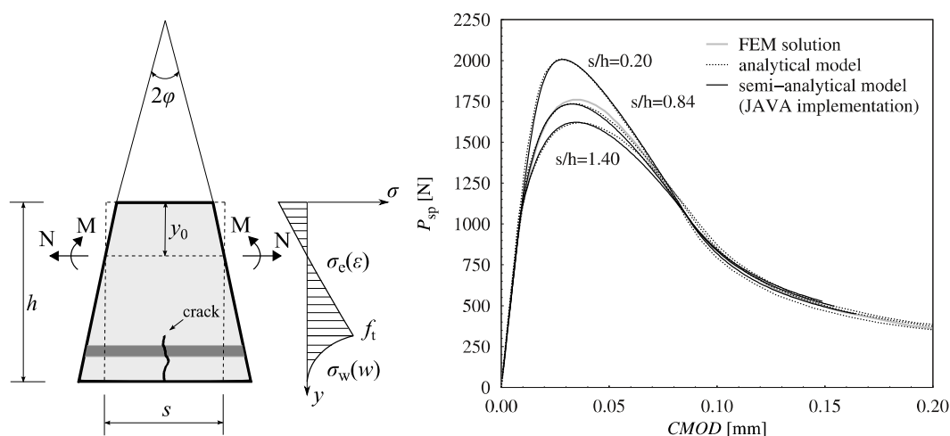
Fig. 1: Loading and deformation of the cracked hinge element with stress distribution (left); comparison of the P -CMOD response of the implemented semi-analytical model with data of FEM and analytical solution originally published by Østergaard (2003)
