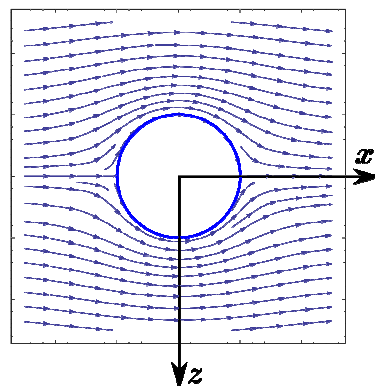
Figure 2. Potential flow in a horizontal plane around a vertical cylinder.
