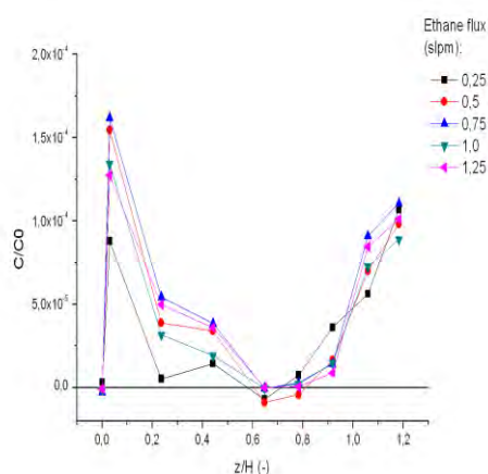
Figure 2: Windward side concentration
