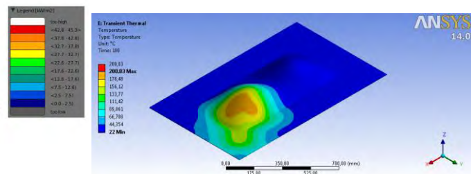
Fig. 4. ANSYS – temperature [2]
