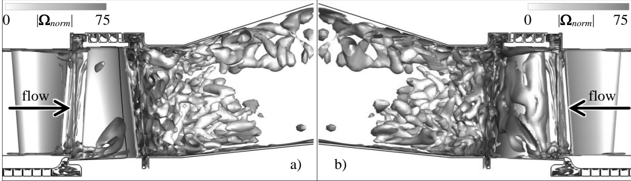
Fig. 4: Structure of vortices behind the axial turbine stage – isosurfaces of Q = (\Omega^2 - \mathbf{S}^2) coloured with the normalized vorticity magnitude |\Omega_{norm}| ; view on the pressure side (a) and on the suction side (b) of the rotor blade.
