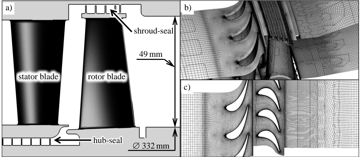
Fig. 2: a) Scheme of the axial turbine stage equipped with the shroud- and hub-seals; b), c) the computational mesh.
