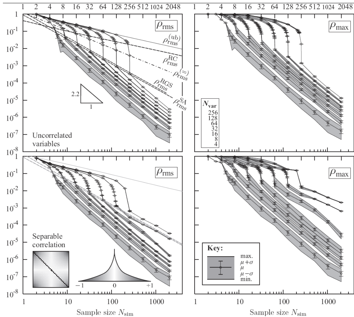
Figure 3. Results of performance study. Top: Uncorrelated variables; Bottom: Separable correlation. Left: \rho_{\text{rms}} ; Right: \rho_{\text{max}} . Bottom left: Image of correlation matrix (absolute values of T_{ij} and distribution of correlation coefficients in \mathbf{T} for the case of studied separable correlation).
