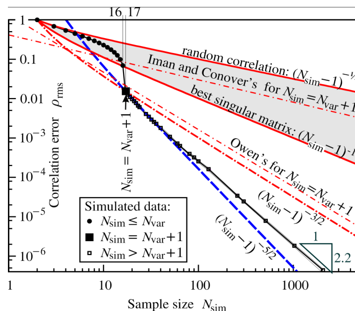
Figure 2. Typical performance plot obtained for N_{var} = 16 . Simulated data (averages are denoted by symbols and a solid line, minima and maxima by thin solid lines) are compared to theoretical bounds and results of other techniques.
