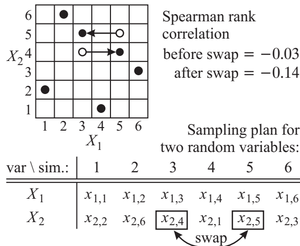
Figure 1. Illustration of a random trial – swap of samples j and k of variable X_2 .
