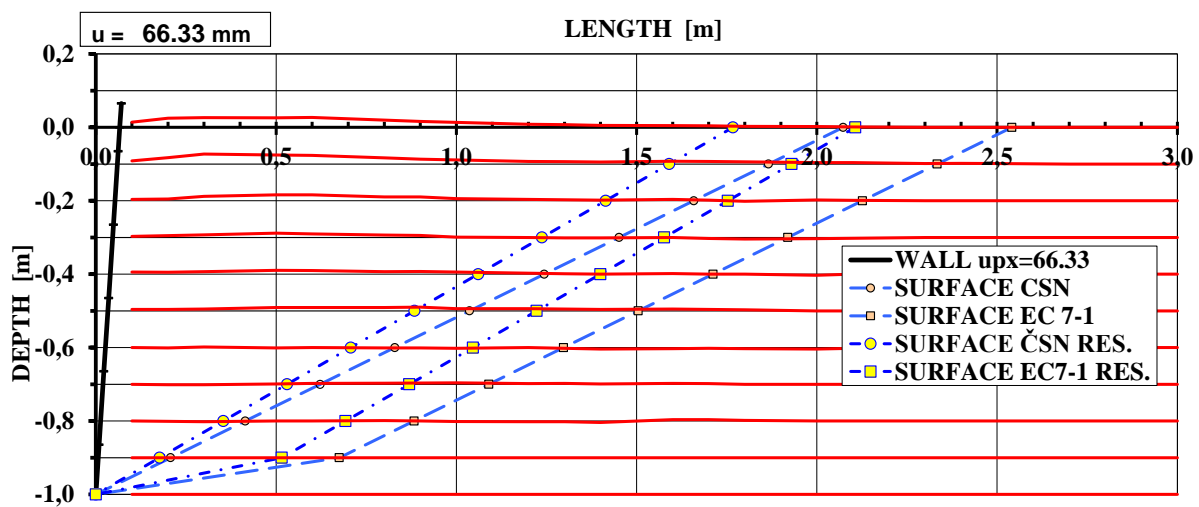
Fig. 3: Measured uplifts and of red strips and slip surface of the sample. Blue dashed lines are theoretically considered shear surfaces for analysis of passive earth pressure according to ČSN 73 0037 and EUROCODE 7-1.
