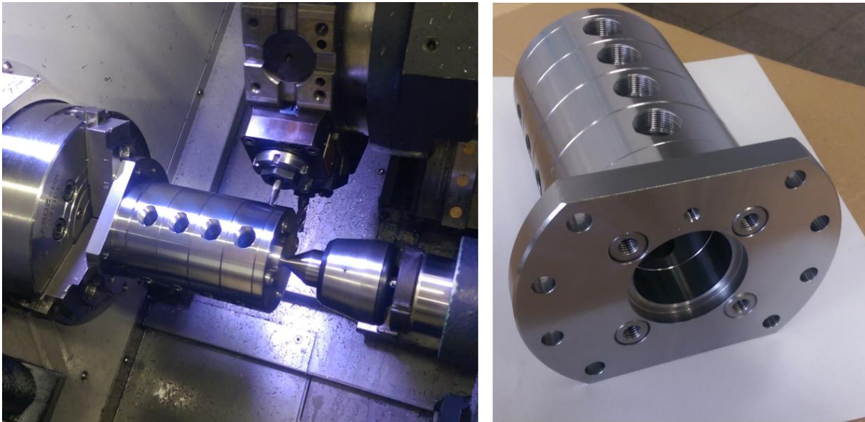
Fig. 3: On the left: the nut cutting by a CNC machining centre, on the right: finished nut without standardized part.
