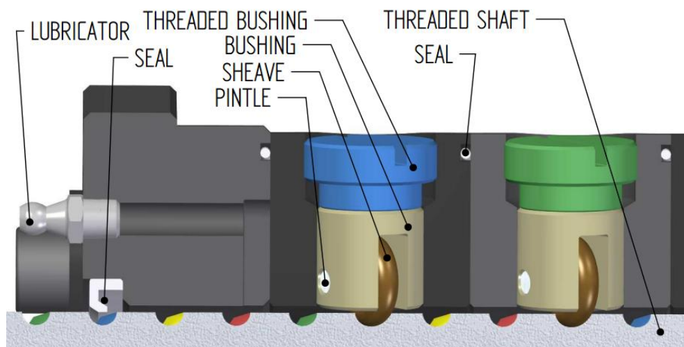
Fig. 2: Detail of shaves inside rings.
