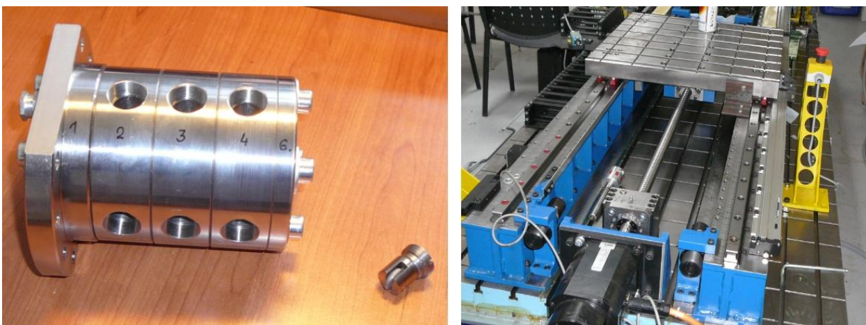
Fig. 4: On the left: the nut with three rings and sheave assembly, on the right: the test bed for measuring of qualities.
