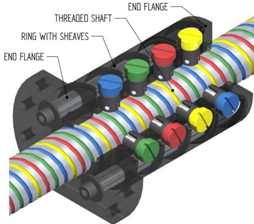
Fig. 1: Section of the motion threaded mechanism.
