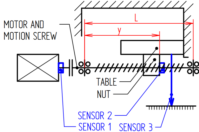
Fig. 5: Schematic picture of the test bed and measurement of the stiffness.
