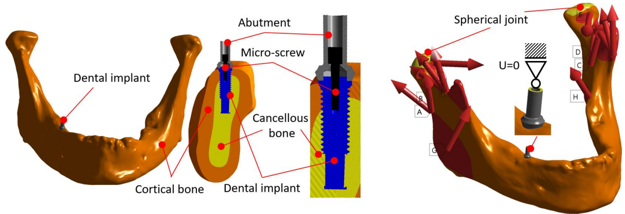
Fig. 1: Geometry model: position of Brånemark dental implant inserted in the mandible.
