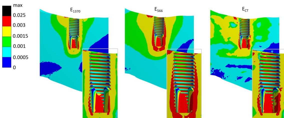
Fig. 3: Strain intensity in cancellous bone.
