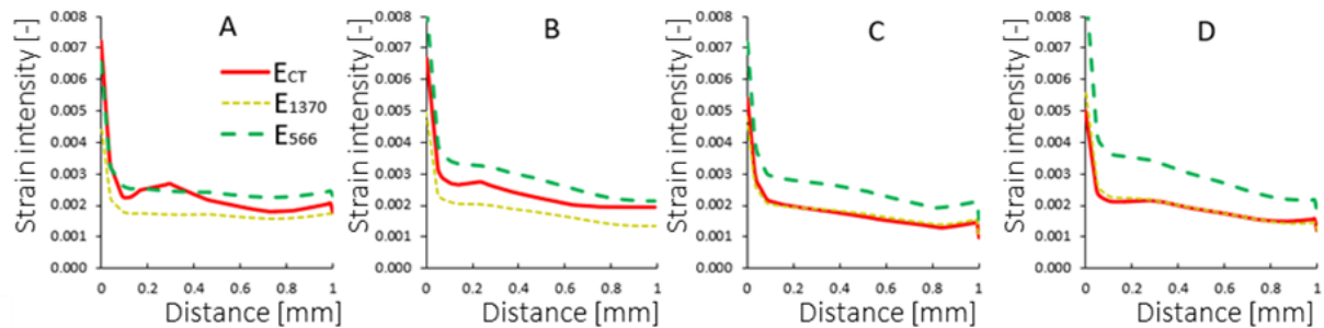
Fig. 4: Strain intensity along paths A, B, C and D.
