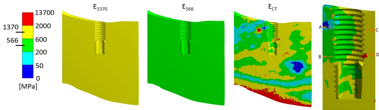
Fig. 2: Three variants of material model of cancellous bone tissue, highlighted paths A-D.
