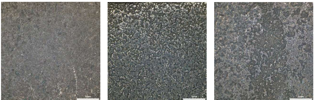
Fig. 3: The turbine blade coating damage during the service life: initial (after GO procedure including ground test: less than 1% coating damage - left), first visual detectable damage (after 520 Flight hours: 13% coating damage - middle), major damage (after 819 Flight hours: 32% coating damage - right)
