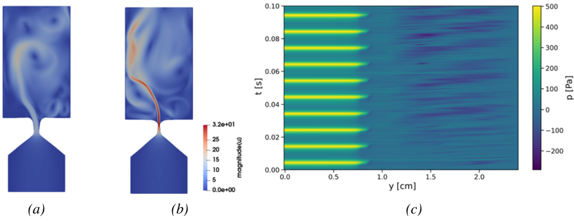
Fig. 3: Velocity magnitude |u| at (a) t = 0.210 and (b) t = 0.21135 , and the pressure along the centerline as a function of time (c).
